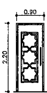
WOODEN DOOR SC=1:50 TYPE-1
